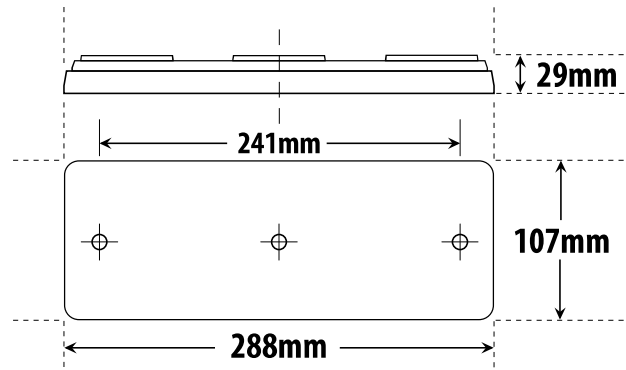
LINE DIAGRAM - BR/OC80ARR &amp; BR/OC80ARW
