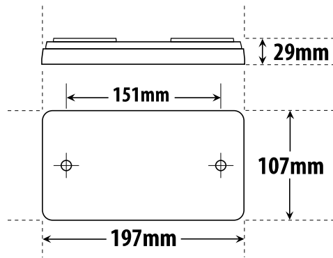
LINE DIAGRAM - BR/OC80AR
