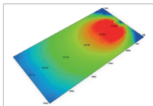
Light Distribution Diagram
