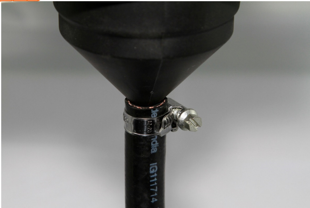
ProVent® 150 with 12mm hose connected and secured with 12-20mm worm drive clamp
