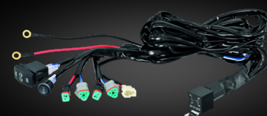
Wiring harness including relay, switches x2, DT connections
