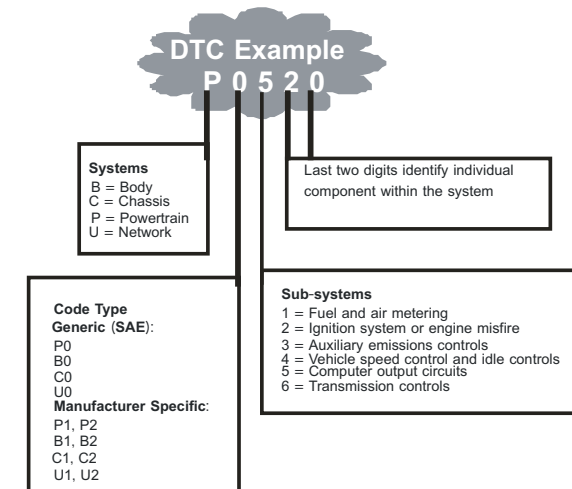
Figure 1-2: Explanation of a diagnostic trouble code.
