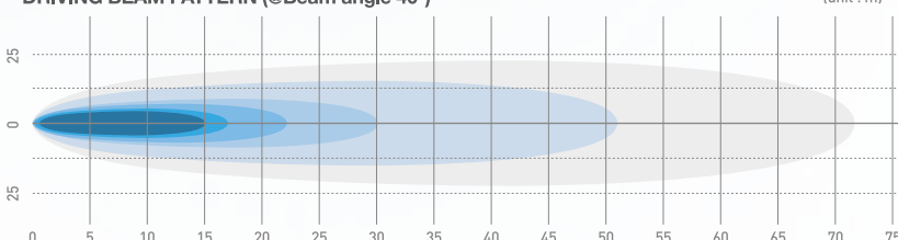
DRIVING BEAM PATTERN (@Beam angle 40°)
