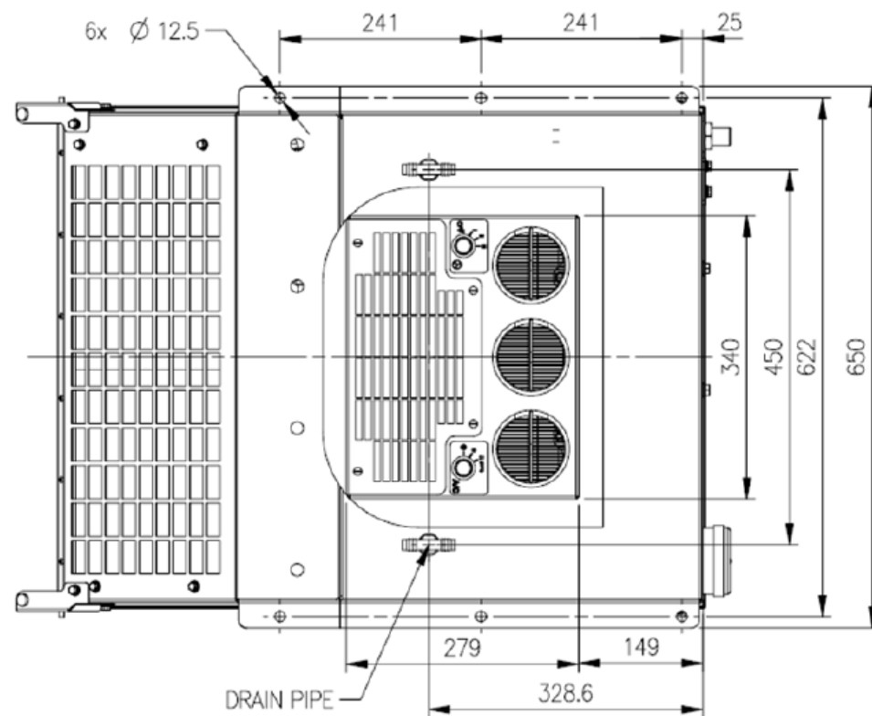
Figure 5-1 Mounting Locations
