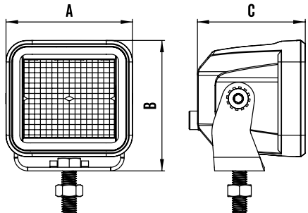
LINE DIAGRAM - RWL4823F
