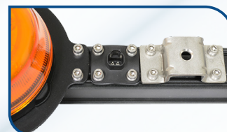
Deutsch connector & bracket for mine flag
